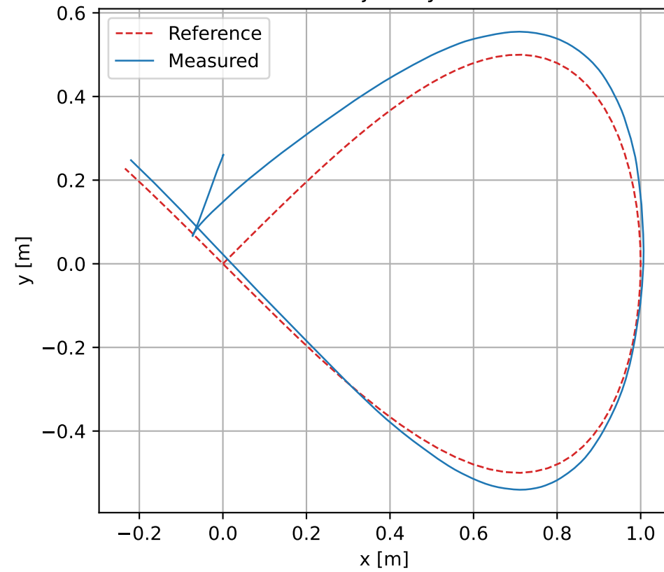
x State
