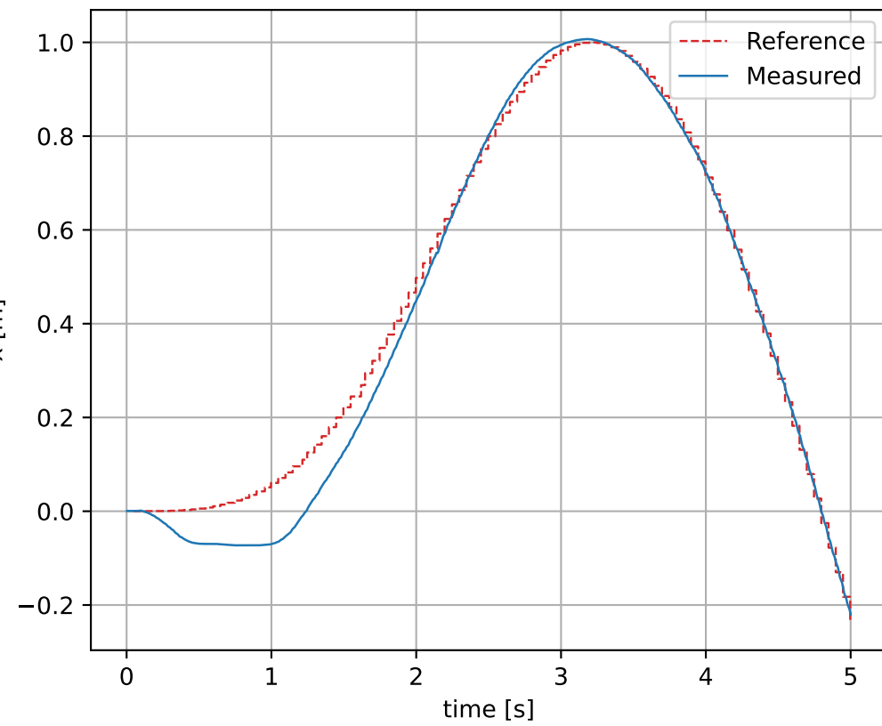
x State
